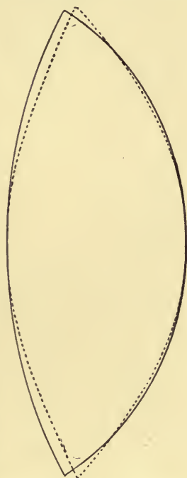
FIG. 110.—Change in the form of the lens during accommodation. The continued line indicates the shape of the lens in a state of repose. The dotted line shows the shape of the lens with seven diopters of accommodation (Tscherning).
